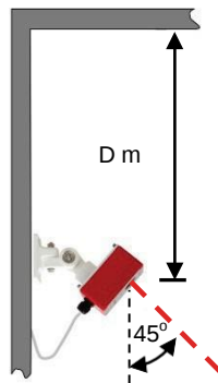
Figure 7. Mounting Clearance
