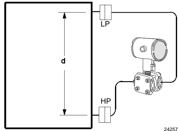
Figure 19- Density, direct acting transmitter configuration
